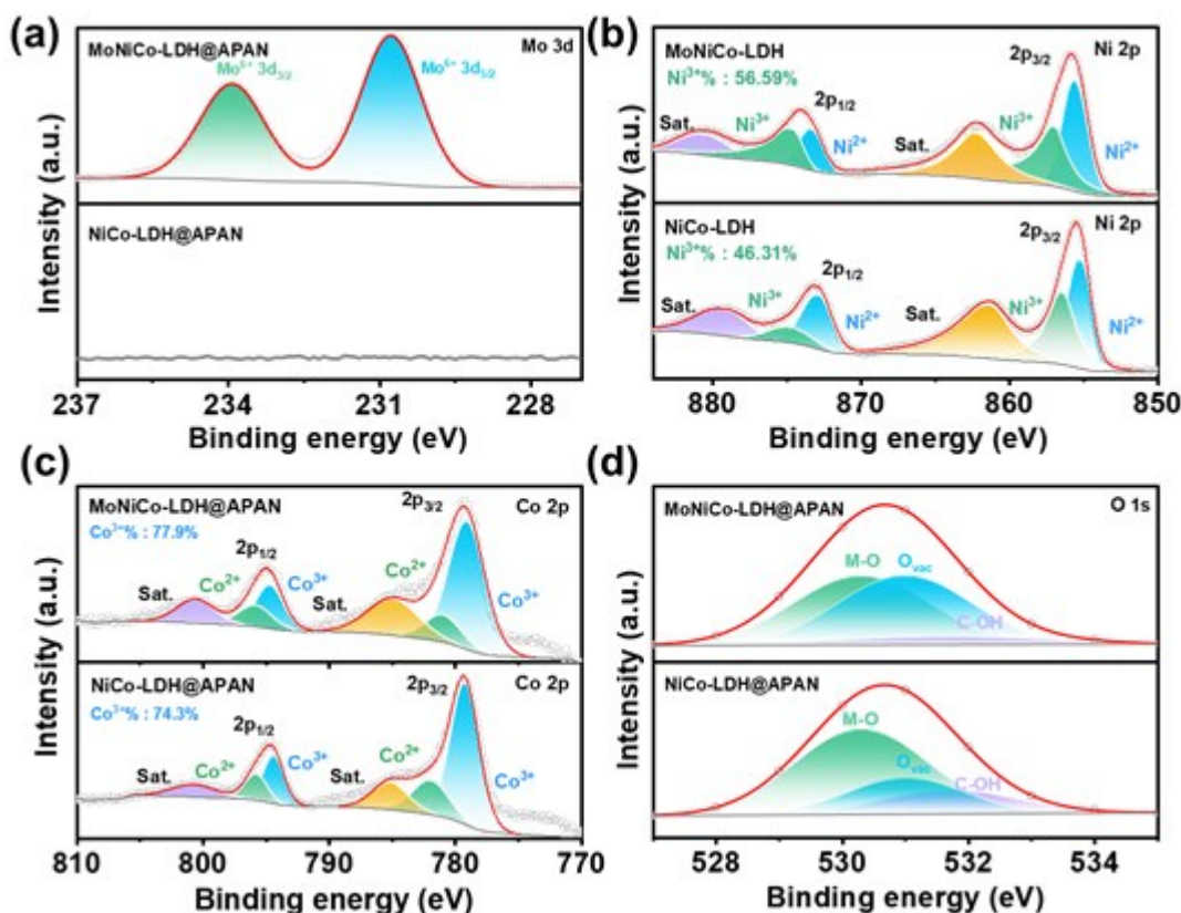
Fig. 3 XPS spectra of (a) Mo 3d, (b) Ni 2p, (c) Co 2p and (d) O 1s of NiCo-LDH@APAN and MoNiCo-LDH@APAN.
