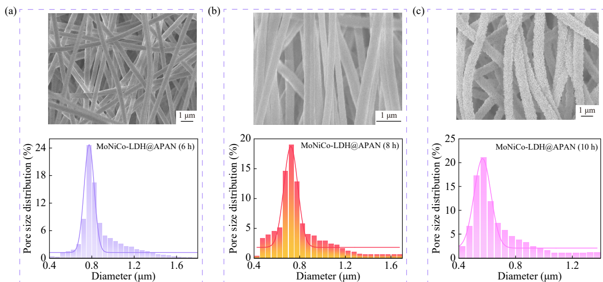
Fig. 2 SEM images and the corresponding pore size distributions of (a) MoNiCo-LDH@APAN (6 h), (b) MoNiCo-LDH@APAN (8 h) and (c) MoNiCo-LDH@APAN (10 h).
