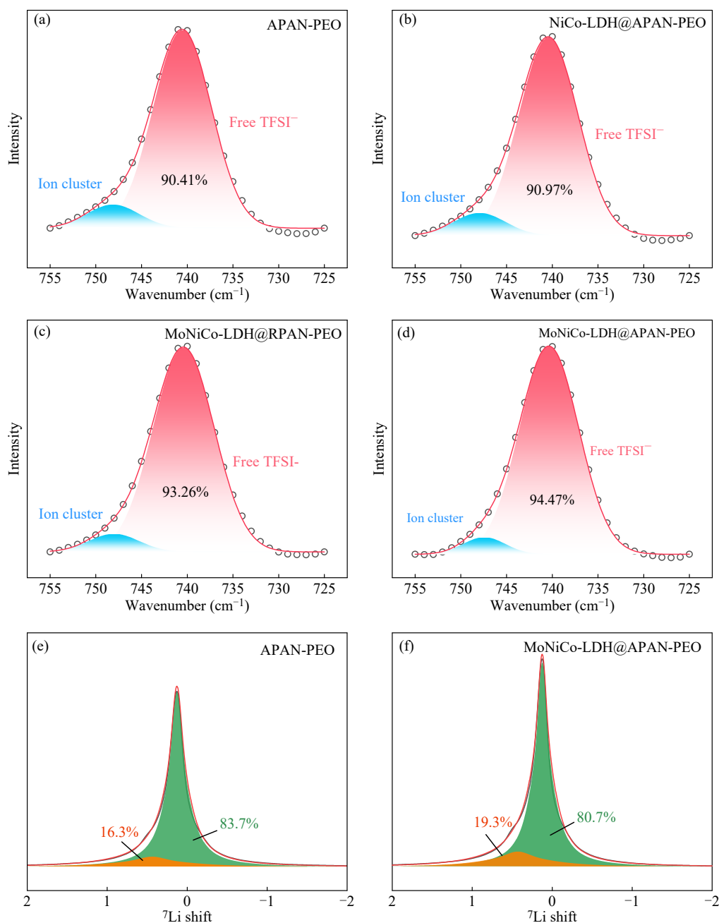
Fig. 6 (a-d) FTIR spectra of different composite solid electrolytes (CSEs) in the range of 725–755 \text{cm}^{-1} ; (e, f) 7 Li-NMR spectra of APAN-PEO and \text{MoNiCo-LDH@APAN-PEO} .
