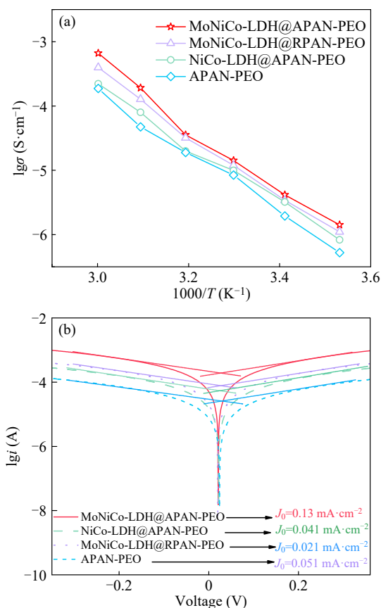
Fig. 7 (a) Ionic conductivities of different CSEs at 10–60 °C; (b) Tafel plots and exchange current density of Li||CSEs||Li based on the LSV tests at -0.35–0.35 V.
