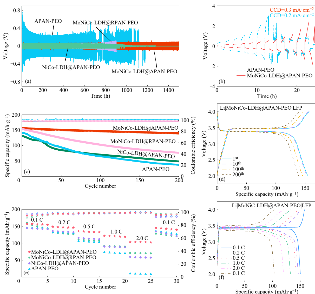
Fig. 9 Electrochemical performance of the cells coupled with different electrolytes. (a) Cycling performance of Li||Li symmetric cells; (b) CCD tests; (c) Long cycle performance of Li||LFP full cells at 0.5 C at 60 °C, and (d) corresponding charge-discharge curves at different cycles; (e) Rate performance of Li||LFP full cells, and (f) corresponding charge-discharge curves at different C-rates.
